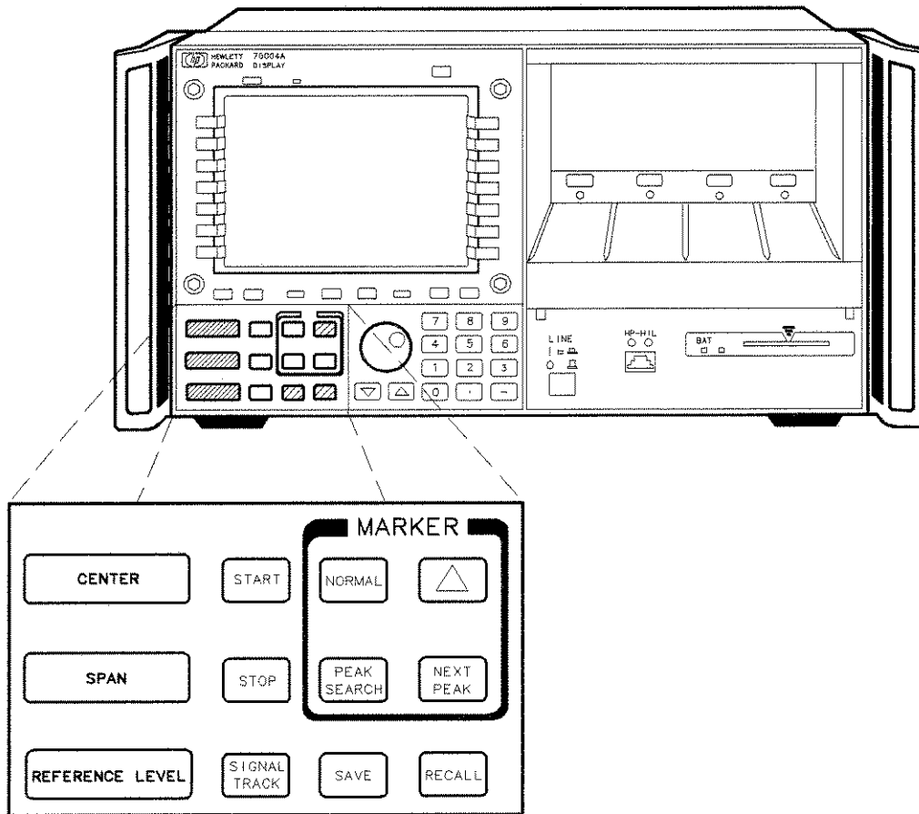
Spectrum Analyzer Instrument Keypad
